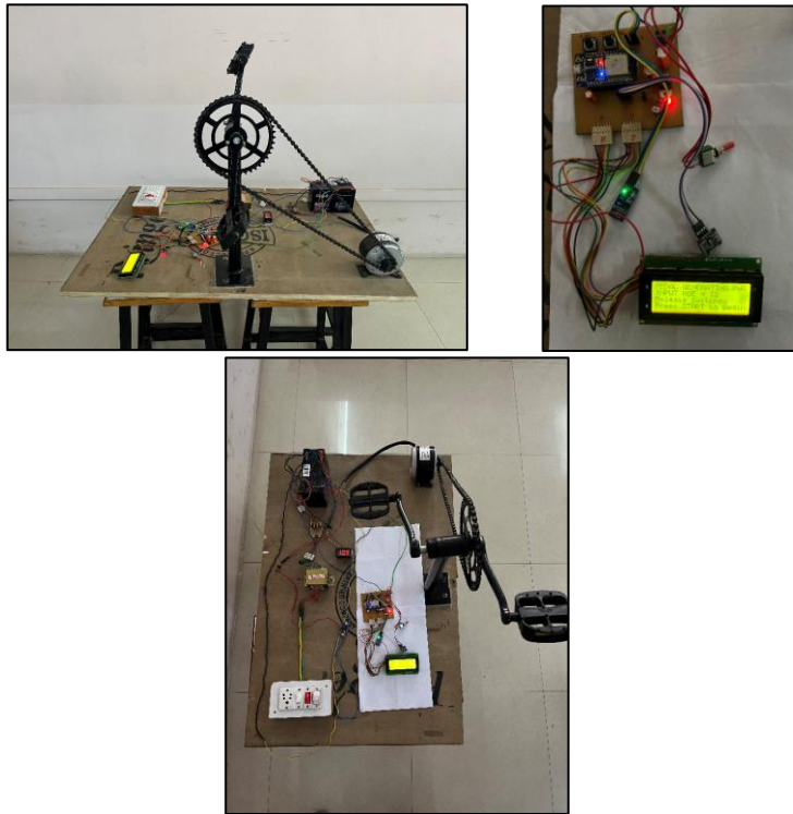
Fig. 7. Images of the prototype
