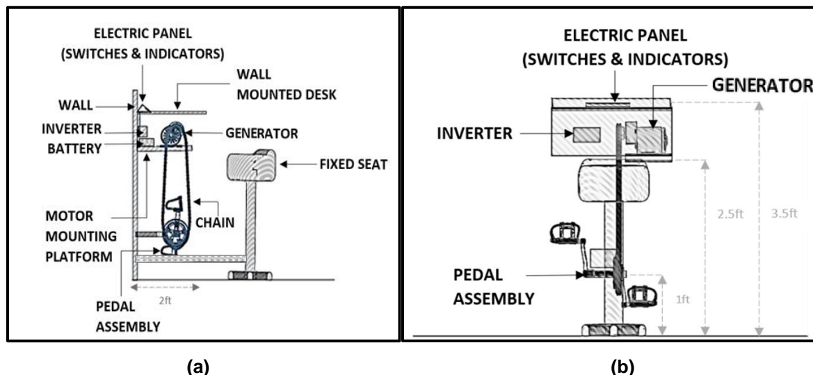
Fig. 1. Pedal's power generation system (a) side view (b) front view
