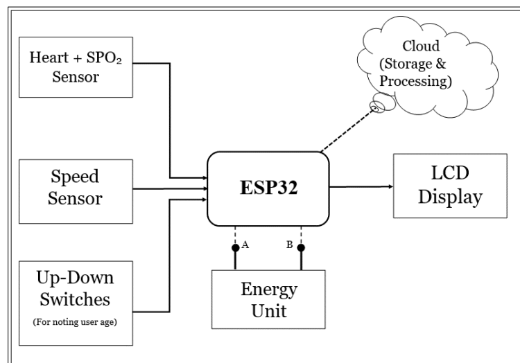
Fig. 6. Block diagram (Part II)
