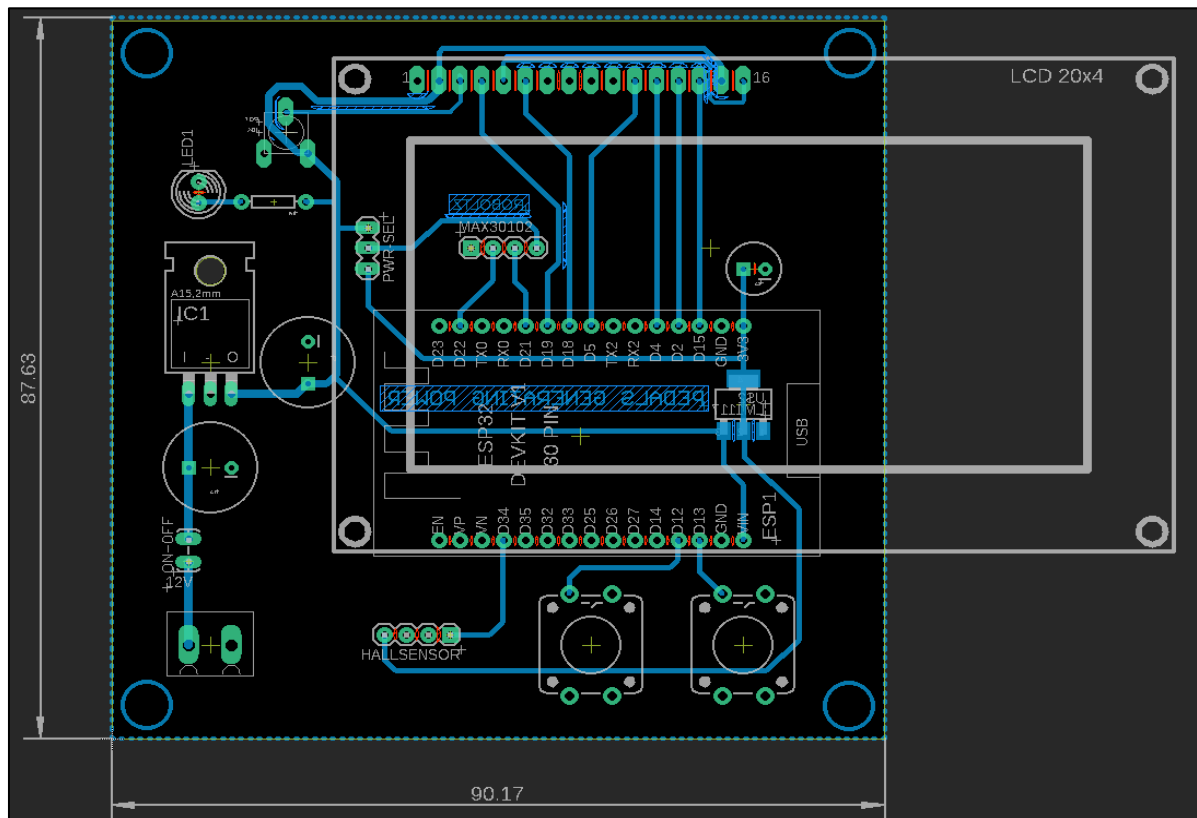
Fig. 5. Health monitoring framework PCB board in Eagle
