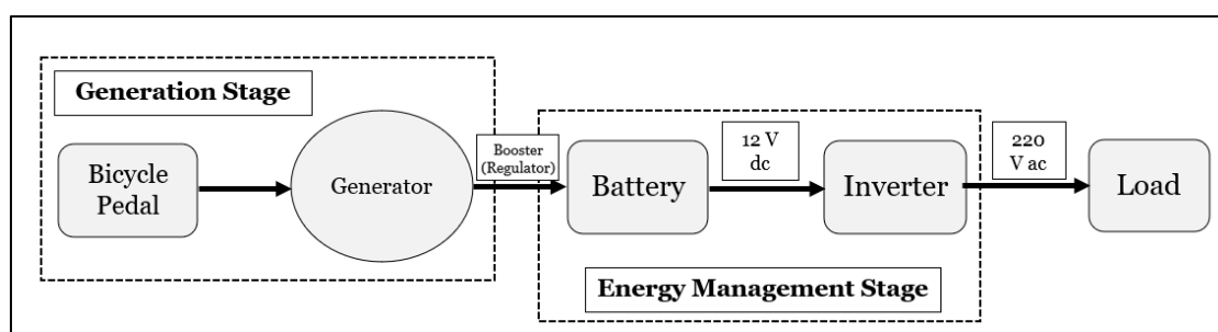
Fig. 2. Block diagram (Part I)
